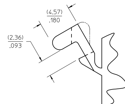
DETAIL 1 .093/(2.36) PREBENT MOUNTING EAR
