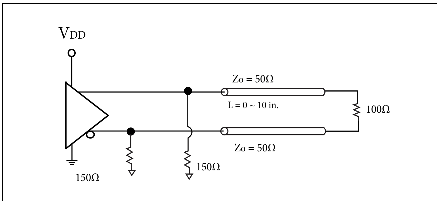
Figure 5. LVPECL output termination
