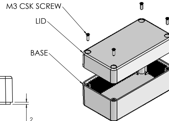
ISO VIEW 1:3
