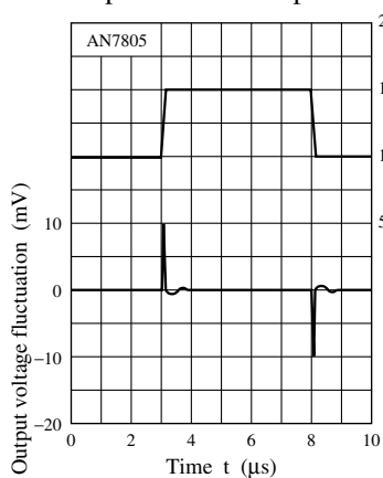
Input transient response
