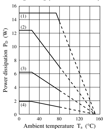
P_D - T_a (AN78xx series)
