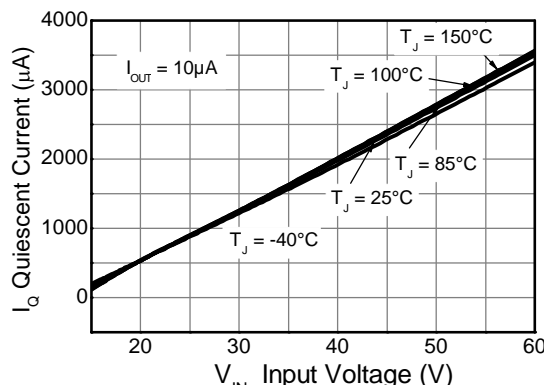
Quiescent Current
