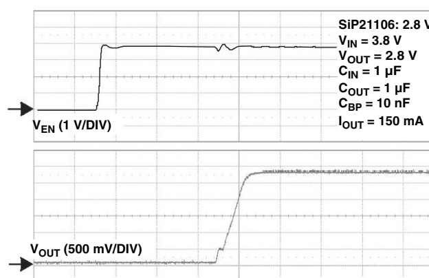
20 μs/DIV Output Voltage Start-Up
