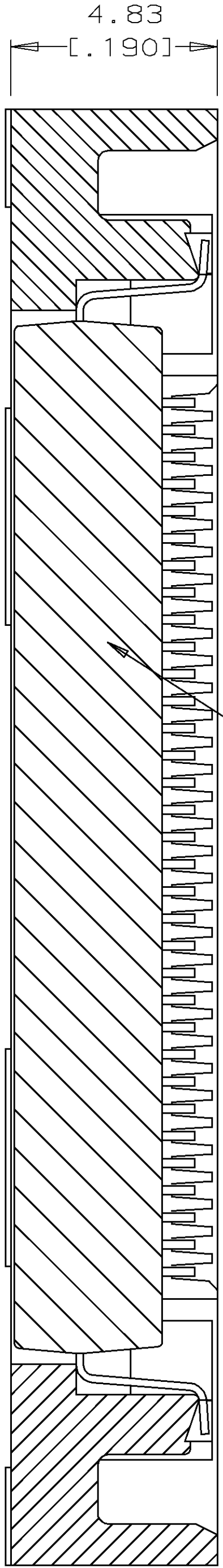
SECTION Z-Z
