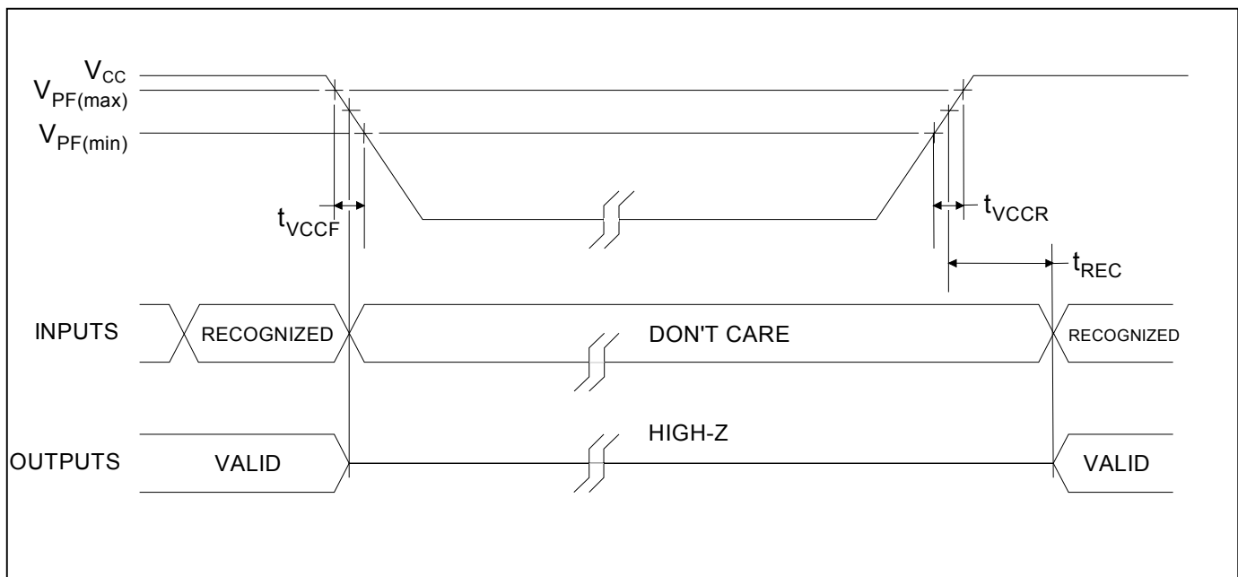
Figure 1. Power-Up/Power-Down Timing
