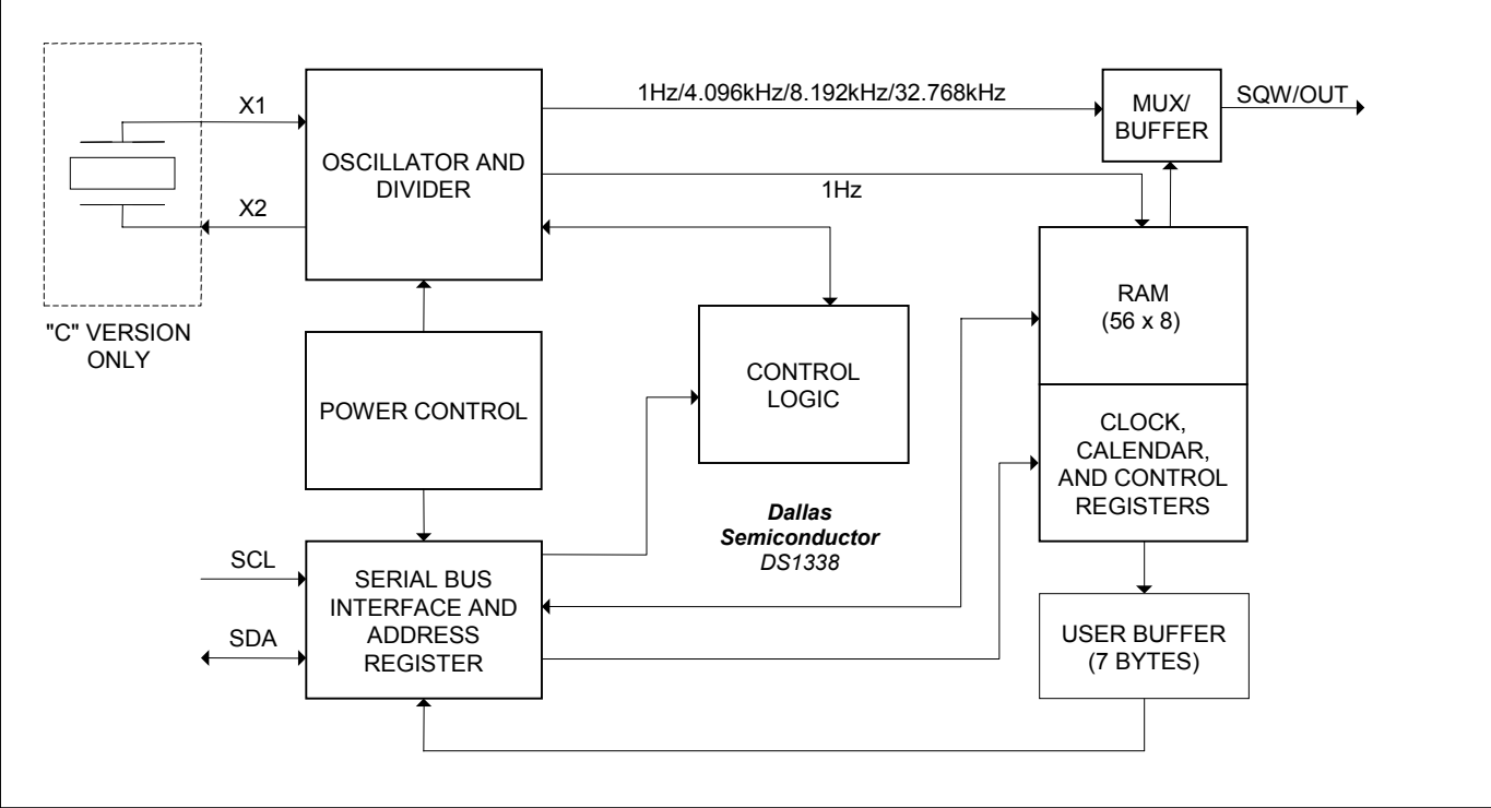
Figure 3. Block Diagram
