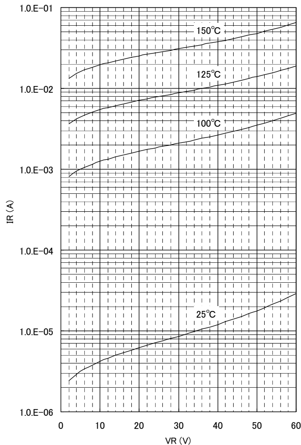
FMW-2156 VR-IR Characteristics
