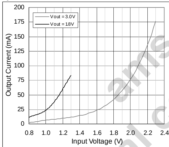
Figure 11. Powersave Threshold vs. V_{IN}
