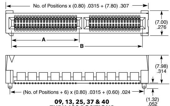
09, 13, 25, 37 & 40 THRU 100 POSITIONS
