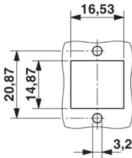
Panel cutout
