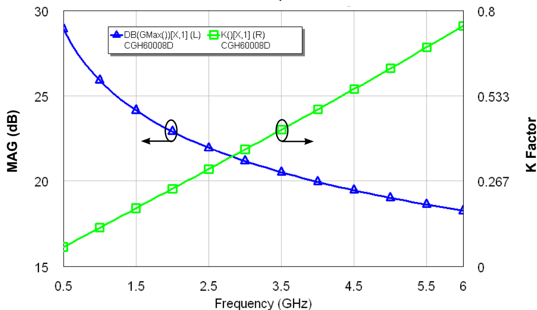
Simulated Maximum Available Gain and K Factor of the CGH60008D
