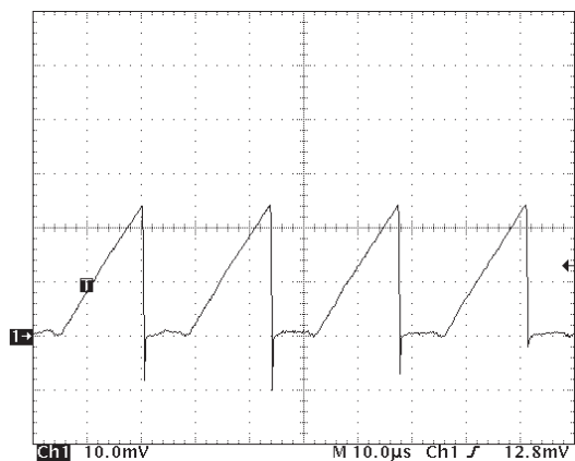
Figure 4. I_SENSE threshold
