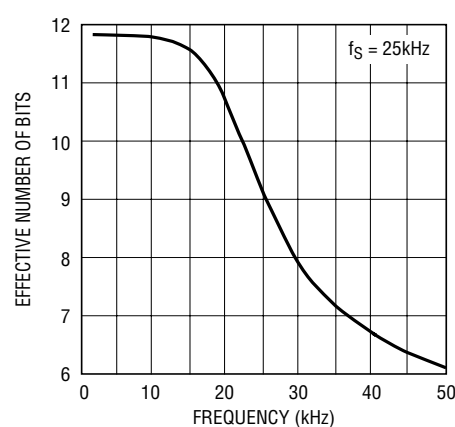
LTC1289 • A1F18
