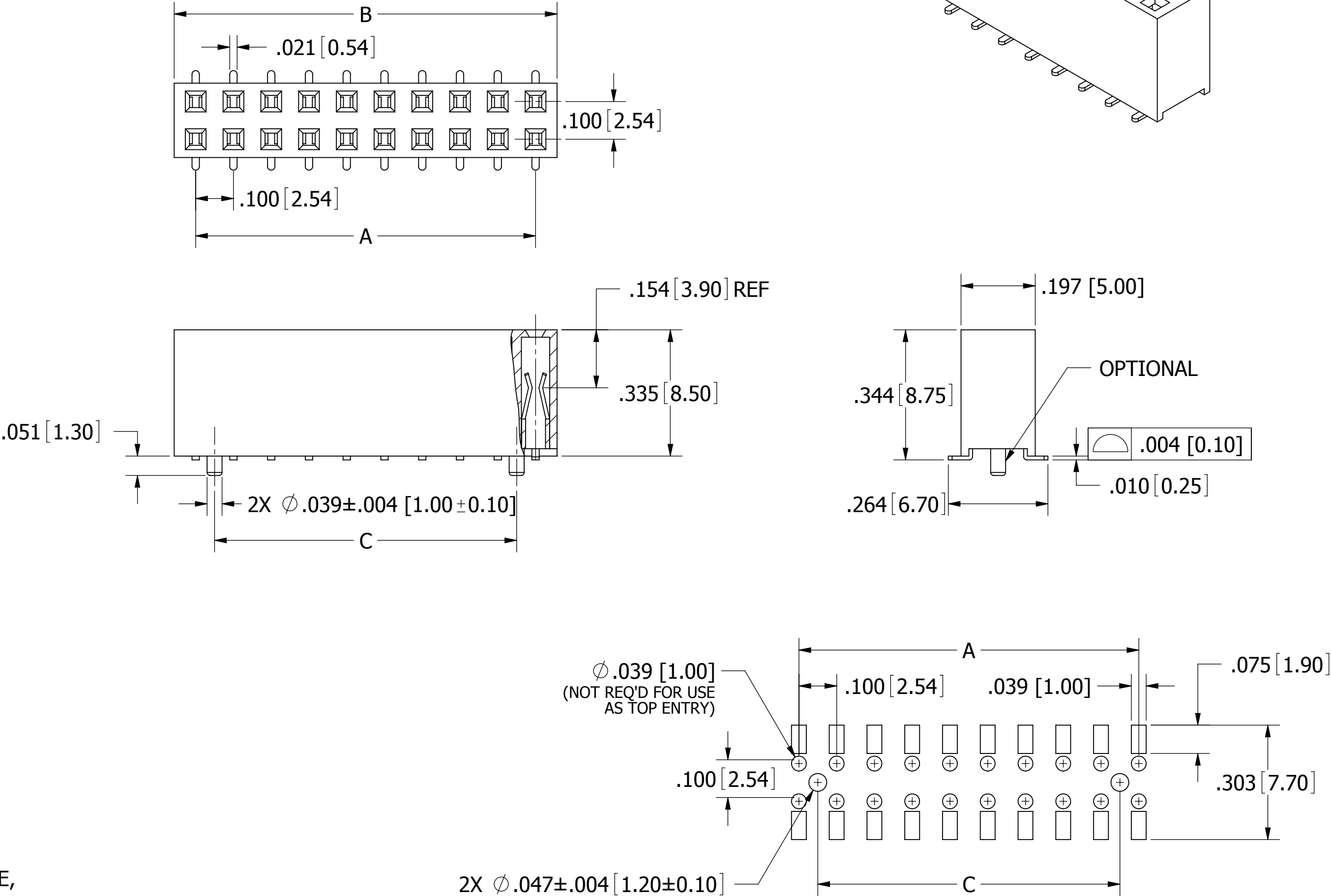
RECOMMENDED PCB LAYOUT
