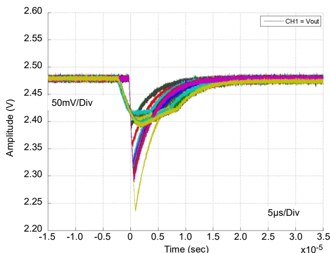
Figure 42. Composite SET Plot for ISL71010B25 at LET 28\text{ V}_{\text{IN}} = 30\text{V} , \text{I}_{\text{OUT}} = 20\text{mA} , \text{C}_{\text{OUT}} = 0.1\mu\text{F} , \text{C}_{\text{COMP}} = 1\text{nF}
