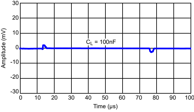
Figure 14. Line Transient with 100nF Load ( \Delta V_{IN} = \pm 500 mV)
