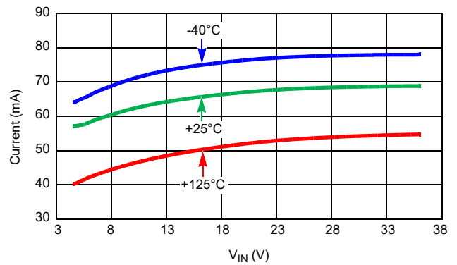
Figure 25. Short-Circuit to V_{IN}
