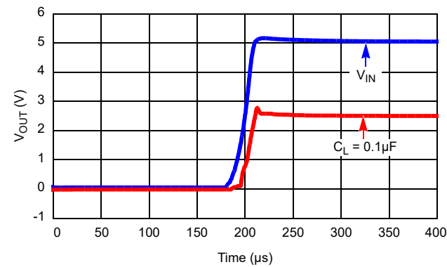
Figure 18. Turn-On Time with 0.1 \mu\text{F}
