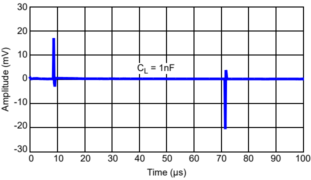
Figure 13. Line Transient with 1nF Load ( \Delta V_{IN} = \pm 500 mV)
