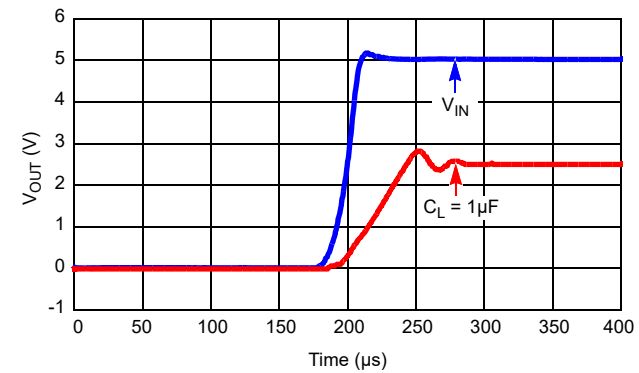
Figure 19. Turn-On Time with 1 \mu\text{F}
