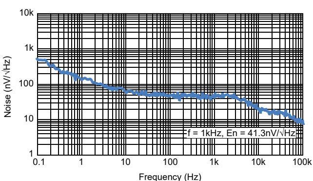
Figure 29. Noise Density vs Frequency (V IN = 5.0V, I OUT = 0mA, C IN = 0.1µF, C OUT = 1µF, COMP = 1nF)
