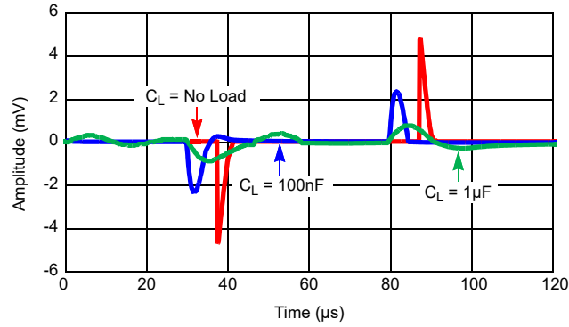
Figure 16. Load Transient ( \Delta I_{LOAD} = \pm 1\text{mA} )
