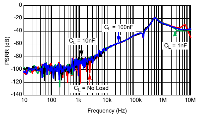
Figure 21. PSRR at Different Capacitive Loads
