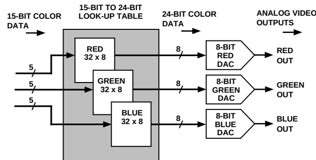
Figure 24. 15-Bit to 24-Bit True-Color Configuration
