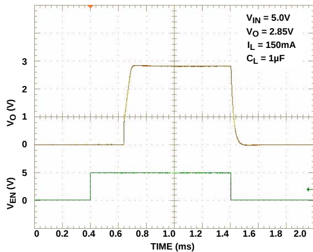
FIGURE 12. TURN-ON/TURN-OFF RESPONSE
