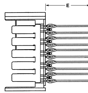
Part Number 120665-1
