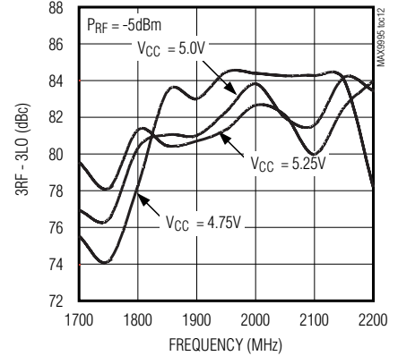
3RF - 3LO vs. FUNDAMENTAL FREQUENCY
