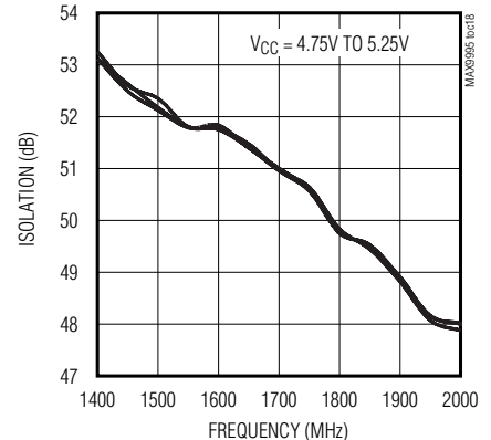
LO SWITCH ISOLATION vs. LO FREQUENCY
