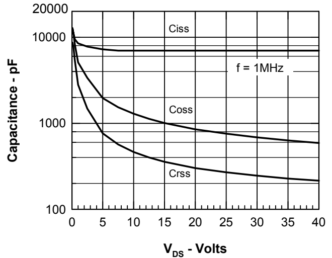
Fig. 7 Capacitance Curves
