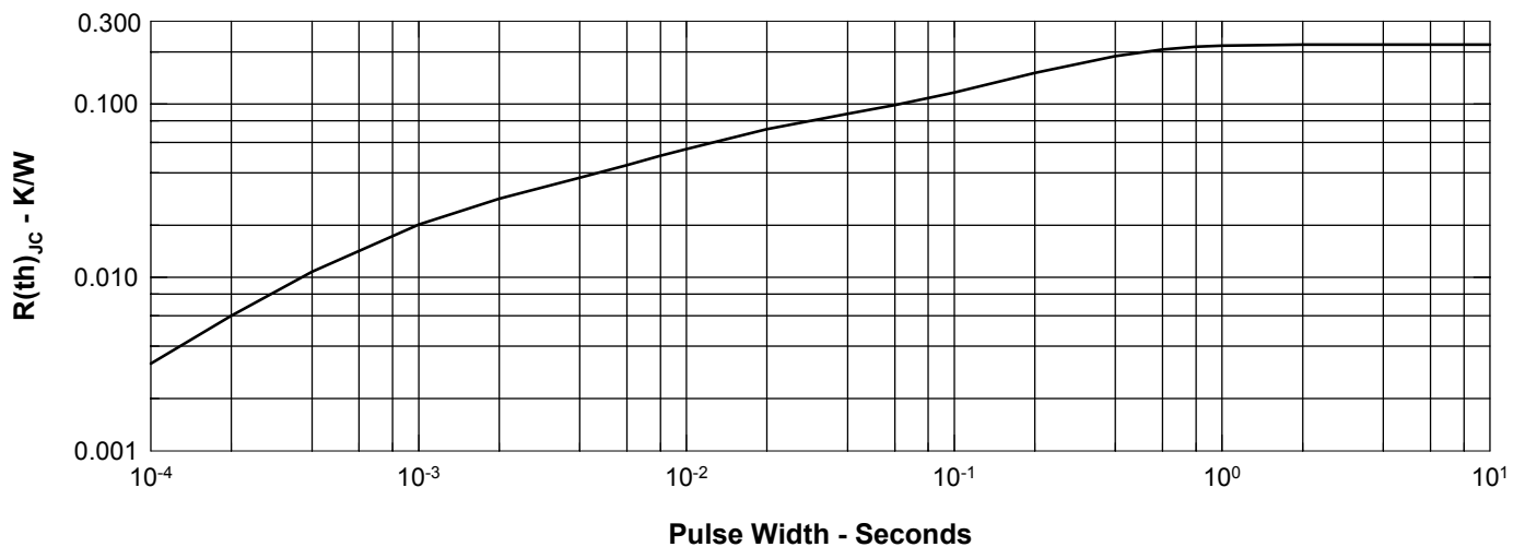
Fig. 10 Transient Thermal Resistance
