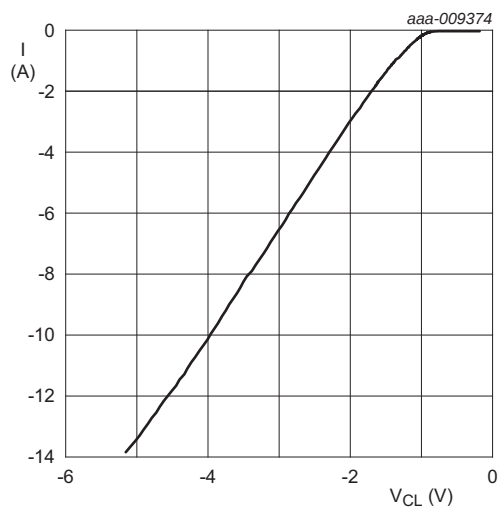
Fig 10. Dynamic resistance with negative clamping; typical values
