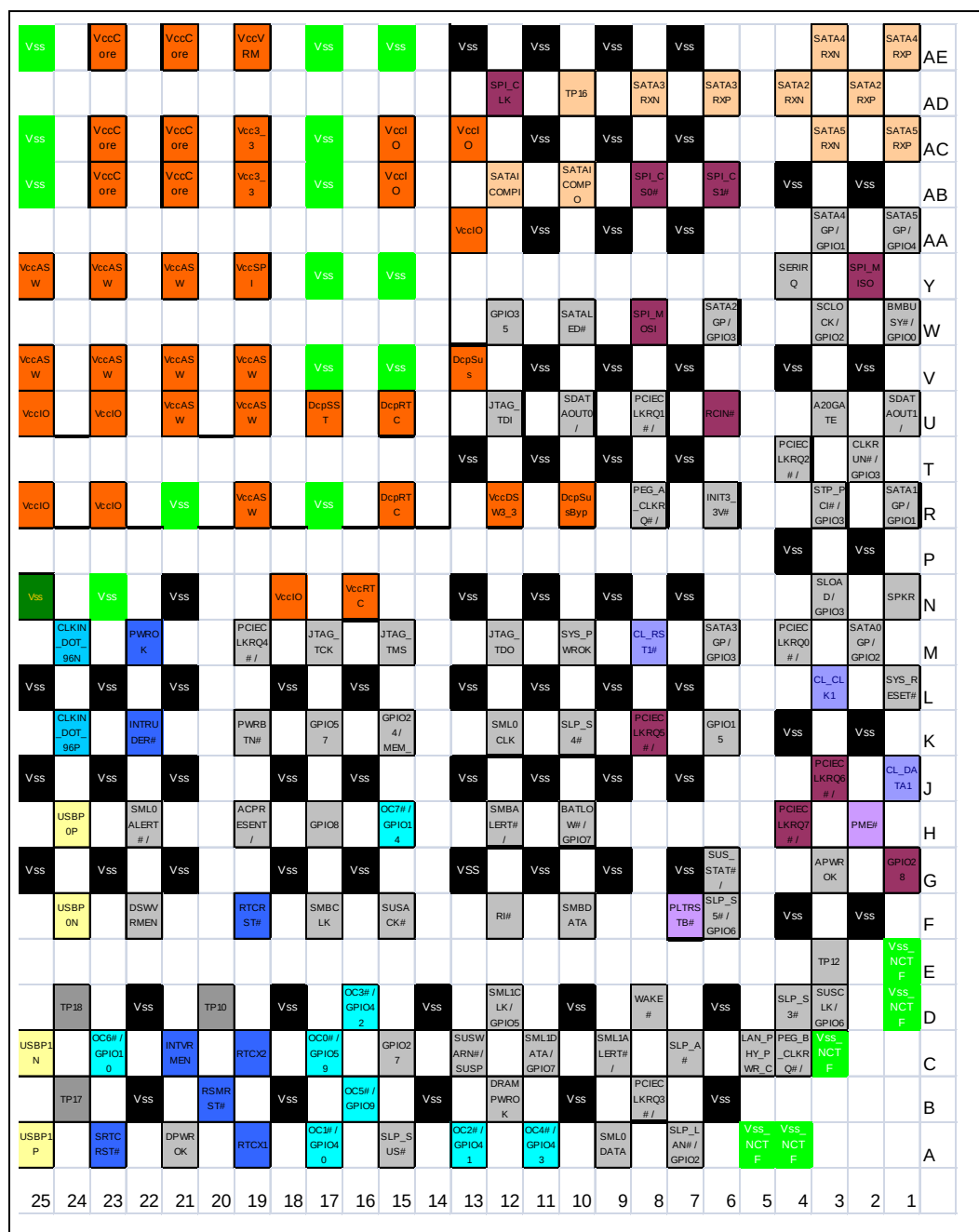
Figure 6-12. Mobile SFF PCH Package (Top View – Lower Right)
