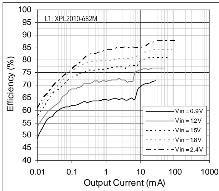
Figure 10: Efficiency vs. Output Current; V_{OUT} = 3.0V
