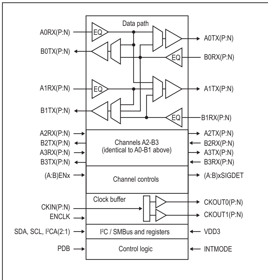
89HP0608R Block Diagram
