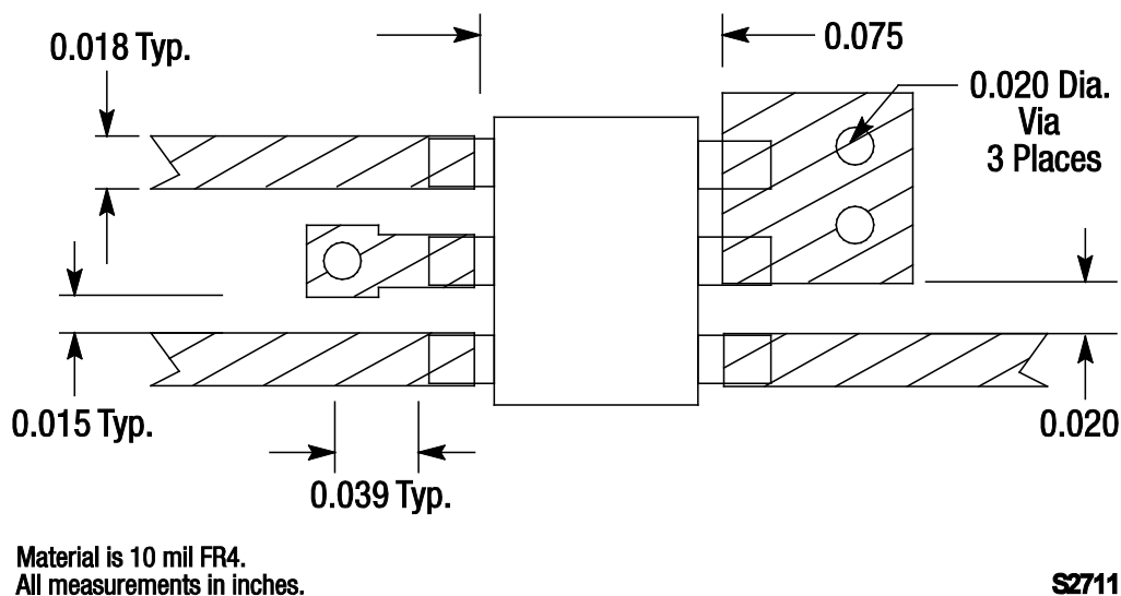
Figure 9. PD18-73/PD18-73LF Recommended Board Layout
