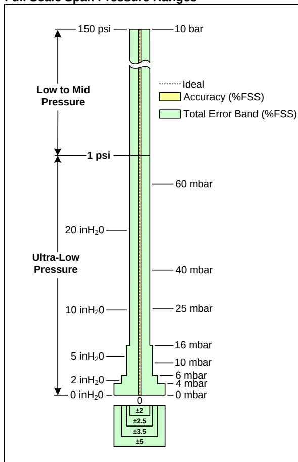
Figure 4. SSC Series Total Error Band Values for Full Scale Span Pressure Ranges
