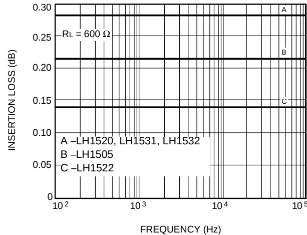
D. Insertion Loss vs. Frequency
