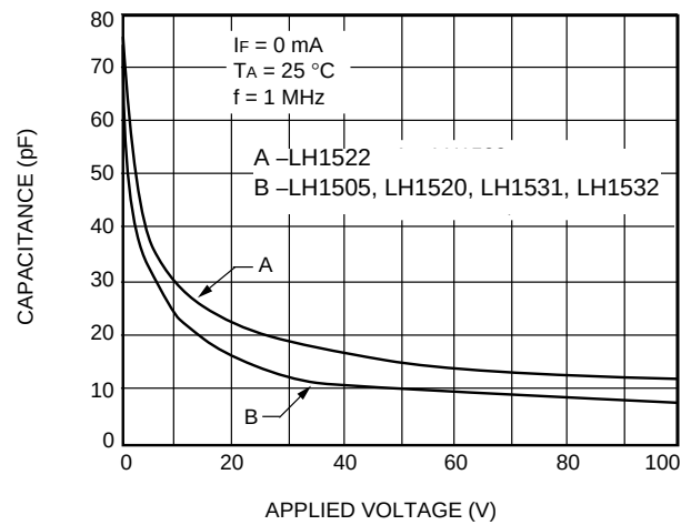
B. Switch Capacitance vs. Applied Voltage
