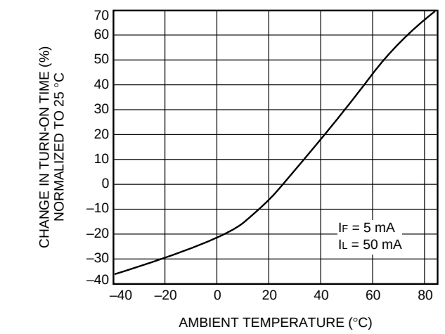
D. Turn-On Time vs. Temperature (LH1544)
