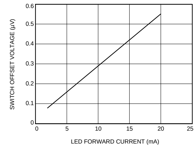
B. Switch Offset Voltage vs. LED Current (LH1544)
