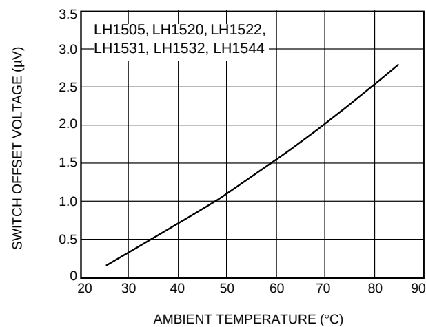
F. Switch Offset Voltage vs. Temperature
