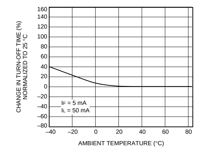
F. Turn-Off Time vs. Temperature (LH1544)
