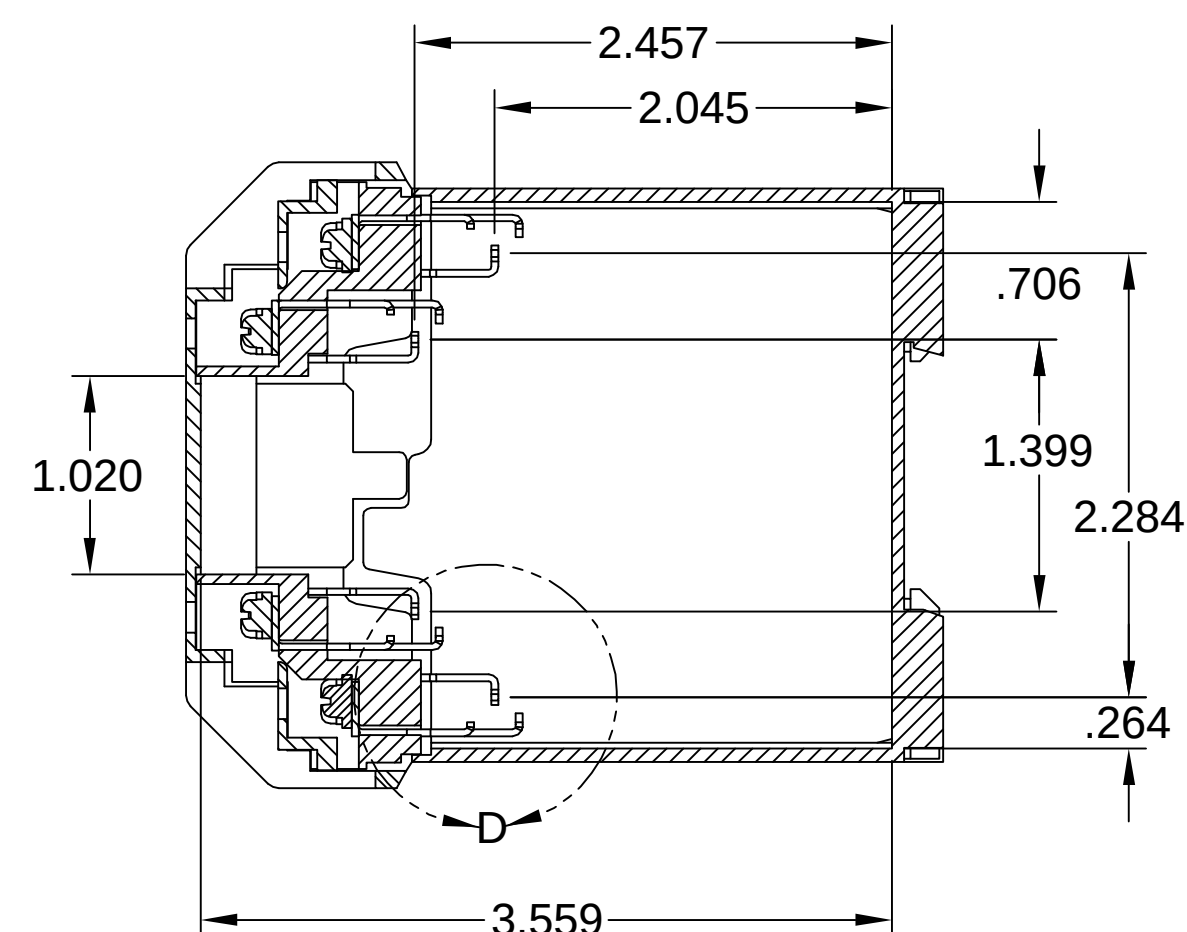
SECTION B-B
