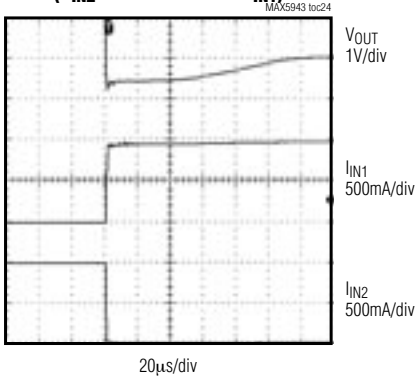
ORing SWITCHOVER WAVEFORM ( V_{IN2} FALLING BELOW V_{IN1} )
