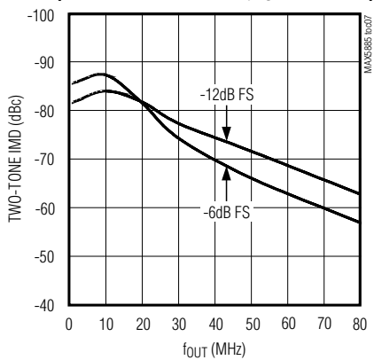
TWO-TONE IMD vs. OUTPUT FREQUENCY (1MHz CARRIER SPACING, f_{CLK} = 200MHz )
