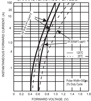
FIG.6- TYPICAL INSTANTANEOUS FORWARD CHARACTERISTICS PER LEG
