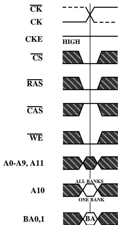
Figure 28. Precharge Command
