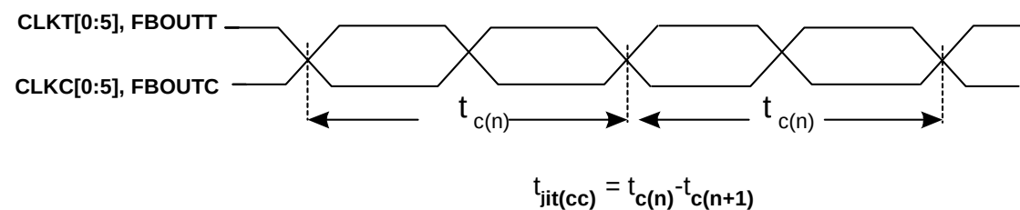
Figure 6. Cycle-to-Cycle Jitter
