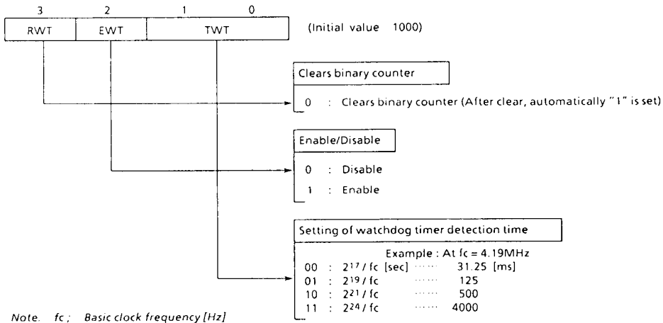
Figure 2-10. Command Register
