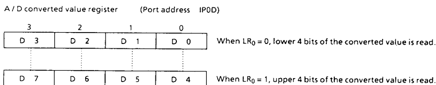
Figure 2-7. A/D converted value register
