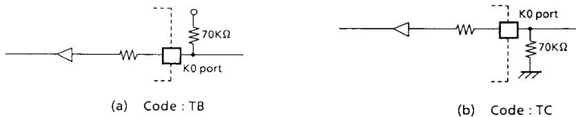
Figure 2. I/O code and external circuitry
