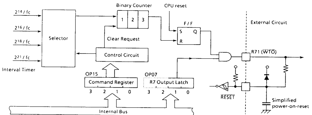
Figure 2-9. Watchdog Timer
