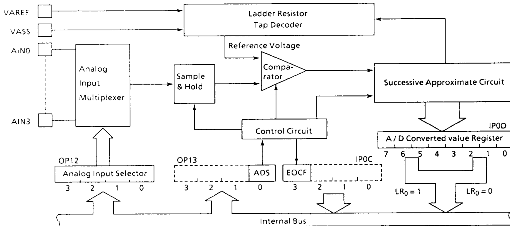
Figure 2-4. Block Diagram of A/D Converter
