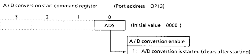
Figure 2-6. A/D conversion start register
