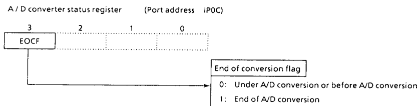
Figure 2-8. A/D converter status register
