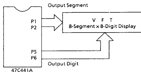
Figure 2-2. Example of driving a VFT
