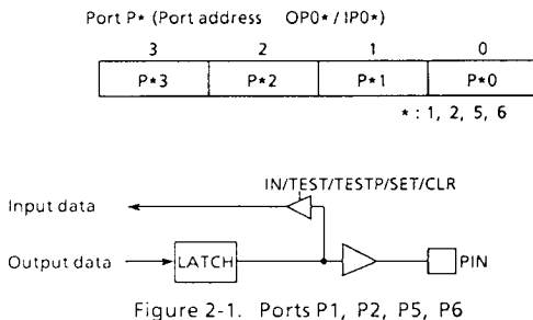
Figure 2-1. Ports P1, P2, P5, P6
