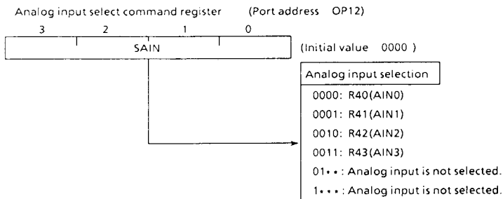
Figure 2-5. Analog input selector
