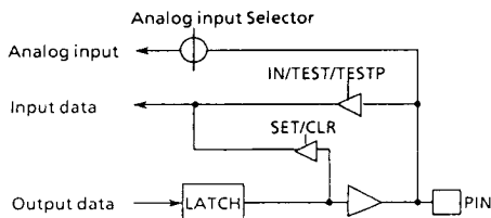
Figure 2-3. Port R4
