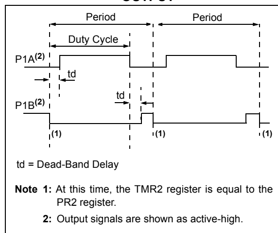
FIGURE 17-4: HALF-BRIDGE PWM OUTPUT
