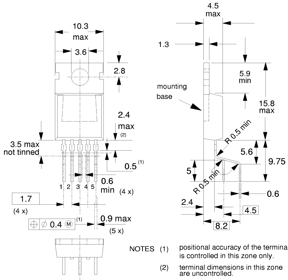
Fig.38. SOT263 leadform 263-01;
