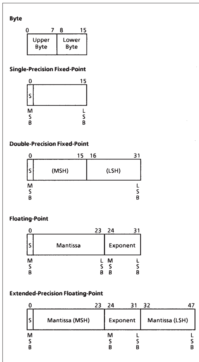
Figure 4: Data Formats
