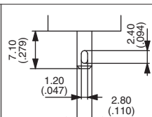
Quick-connect Z
