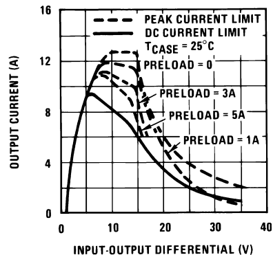
Figure 5-2. Current Limit
