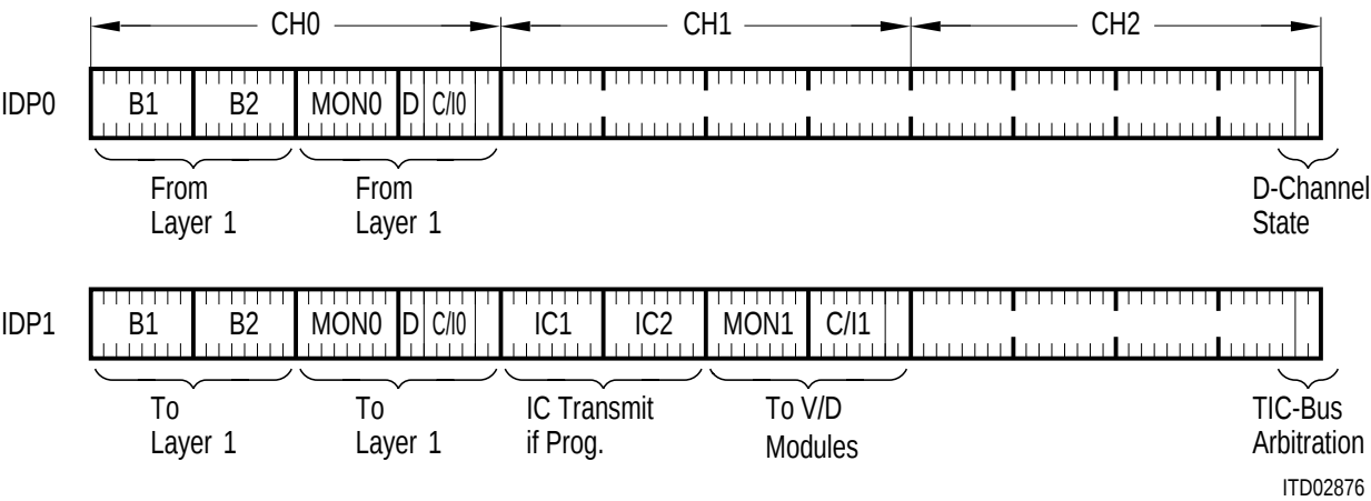
(b) ICC Slave Mode (IDC = 1)
