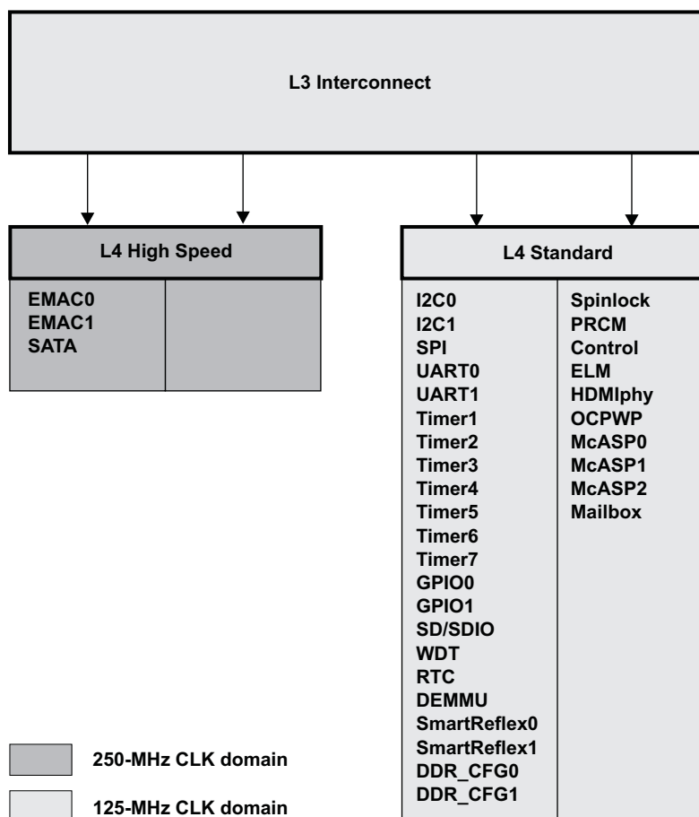
Figure 5-2. L4 Architecture
