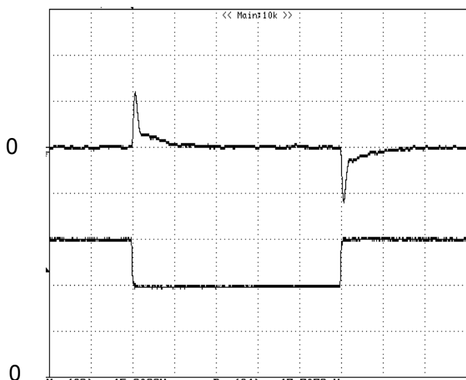
Figure 8: Output voltage response to step-change in load current (75%-50%-75% of I_{o, \max} ; di/dt = 0.1A/\mu s ). Load cap: 10 \mu F tantalum capacitor and 1 \mu F ceramic capacitor. Top Trace: V_{out} (100mV/div, 200 \mu s /div), Bottom Trace: I_{out} (5A/div). Scope measurement should be made using a BNC cable (length shorter than 20 inches). Position the load between 51 mm to 76 mm (2 inches to 3 inches) from the module
