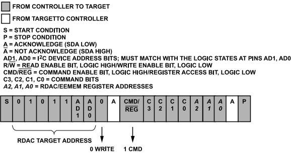
Figure 31. RDAC Quick Command Write (Dummy Write)
