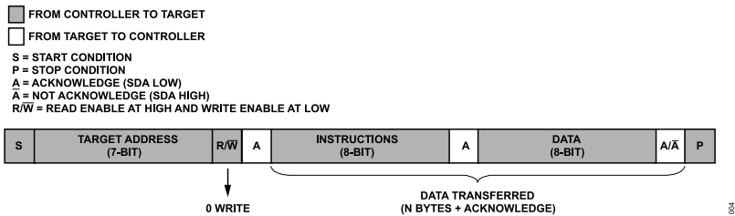
Figure 24. I 2 C—Controller Writing Data to Target
