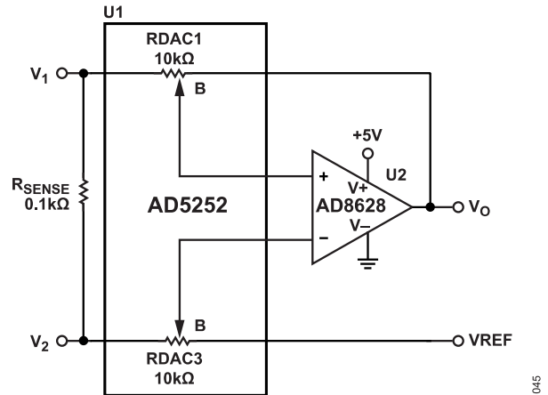
Figure 45. Current-Sensing Amplifier
