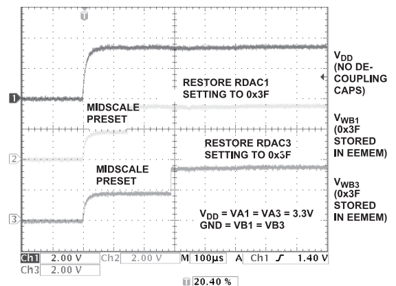
Figure 20. t_{\text{EEMEM\_RESTORE}} of RDAC1 and RDAC3
