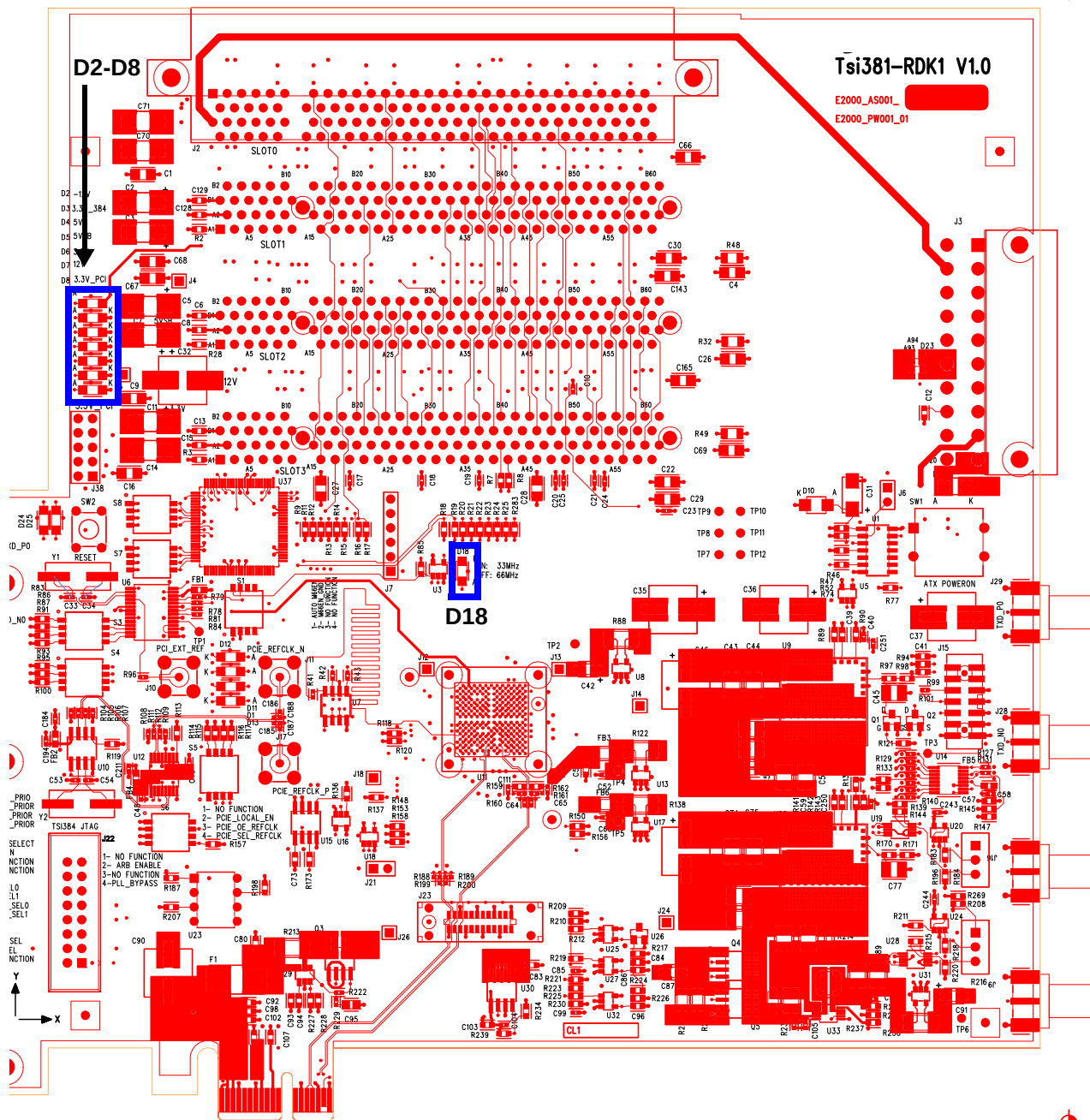
Figure 10: LED Locations
