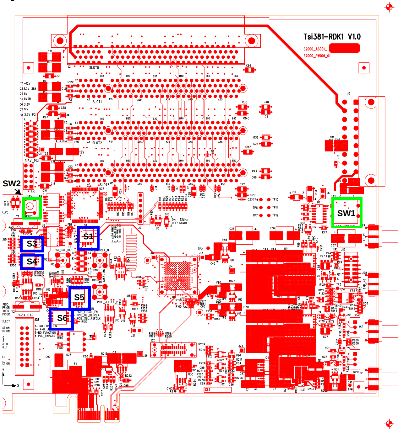
Figure 6: Switch Locations
