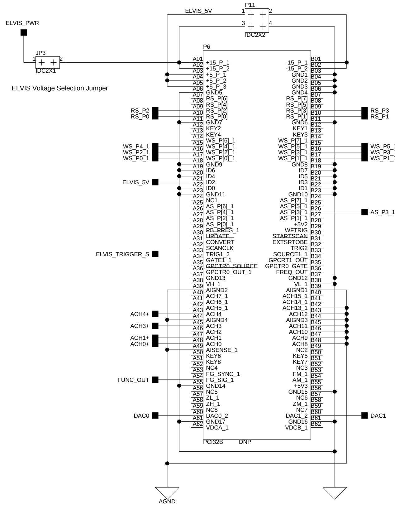
ELVIS CONNECTOR
