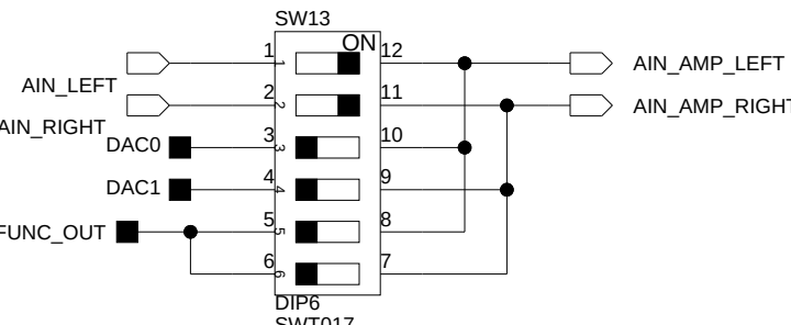
Function Generator Switch
