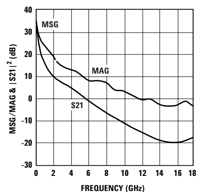
Figure 38. MSG/MAG & |S_{21}|^2 vs. and Frequency at 4.0V/75 mA.
