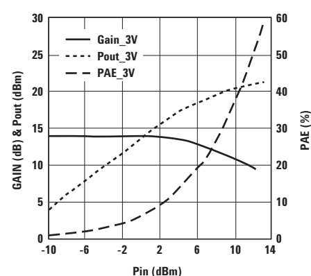
Figure 18. Small Signal Gain/Pout/PAE vs. Pin at V_{ds}=3V and Freq = 2 GHz.
