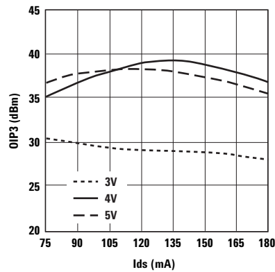
Figure 31. OIP3 vs. I_{ds} and V_{ds} at 2.4 GHz.
