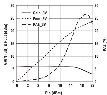
Figure 24. Small Signal Gain/Pout/PAE vs. Pin at V_{ds}=3V and Freq = 5.8 GHz.
