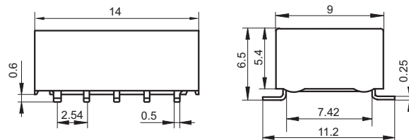
Standard SMT type
