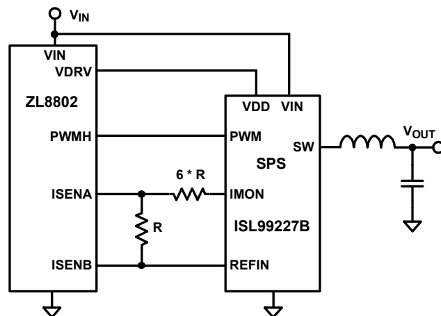
FIGURE 7. SPS CURRENT SENSING
