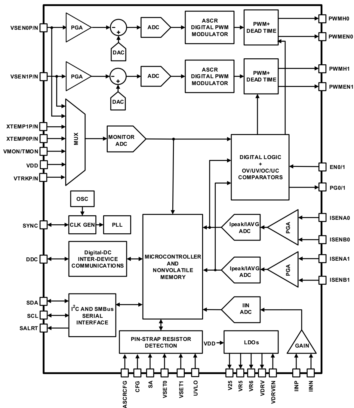
FIGURE 2. BLOCK DIAGRAM
